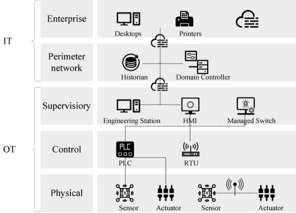
Figure 2: Open-source visual artefact from [6] depicting the SWaT testbed.
